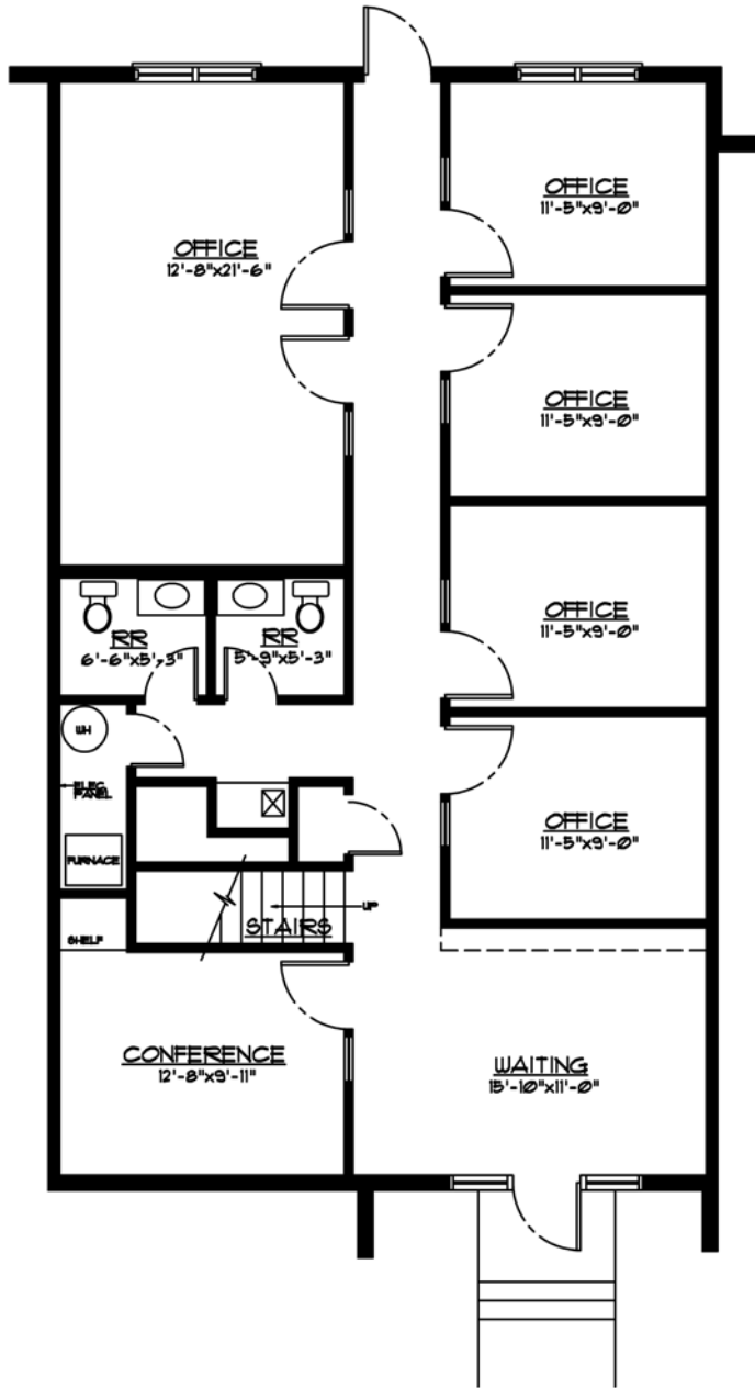
FIRST FLOOR PLAN NOT TO SCALE
