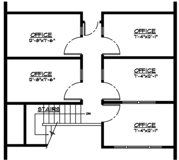
SECOND FLOOR PLAN NOT TO SCALE
